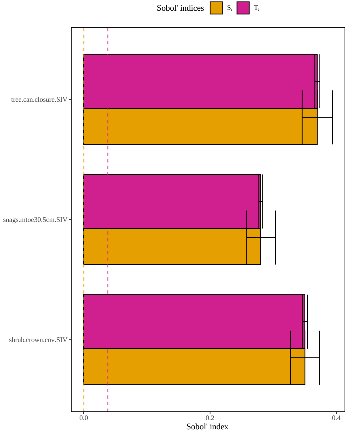
Figure 4. Results of a sensitivity analysis for the lewiswoodpeckerSummerDeciduousDesertic model based on an arithmetic mean structure. Dashed lines represent baseline numerical approximation error for S_i and T_i ( i.e. , dummy variables).
